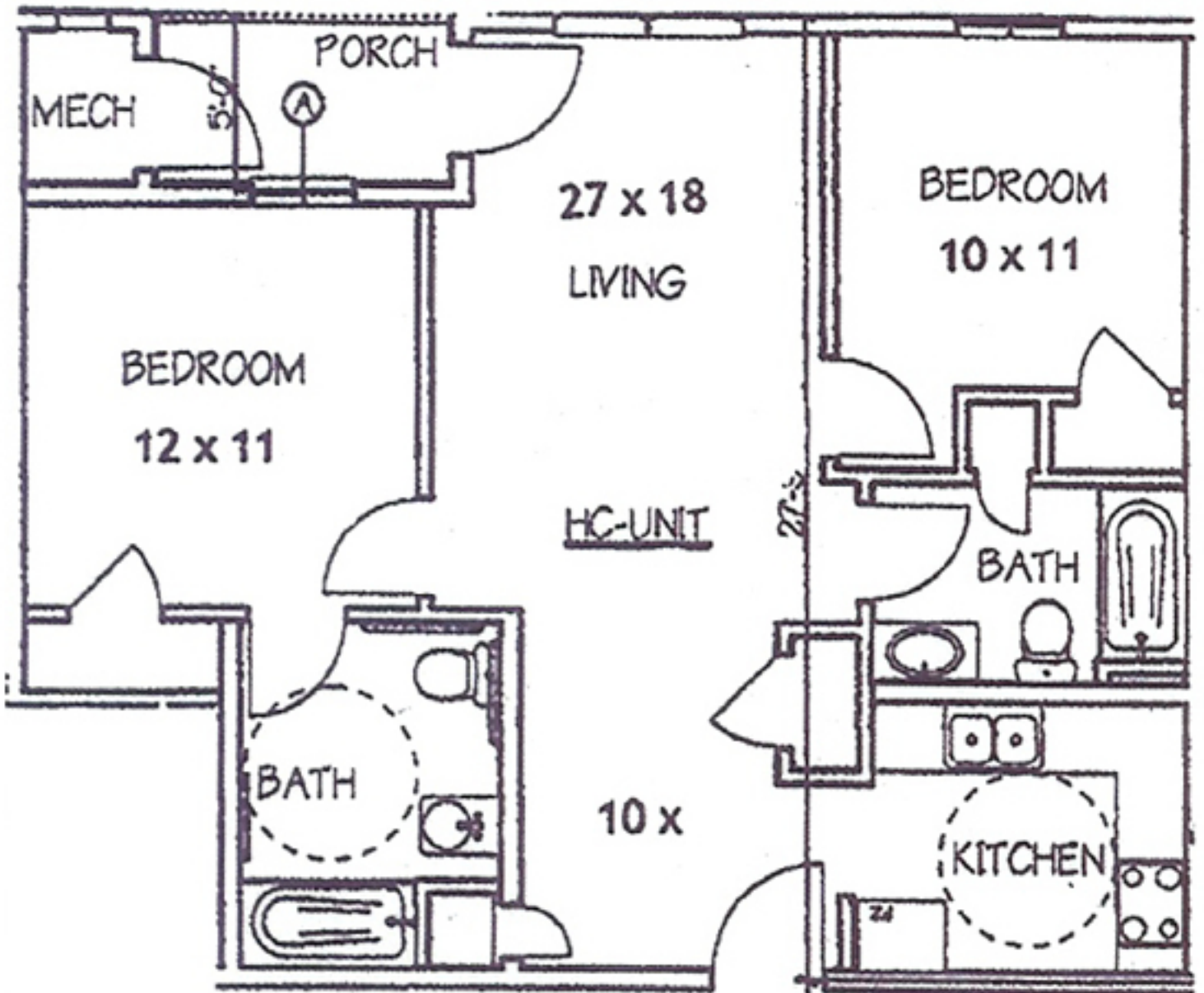
2 BEDROOM / 2 BATH
